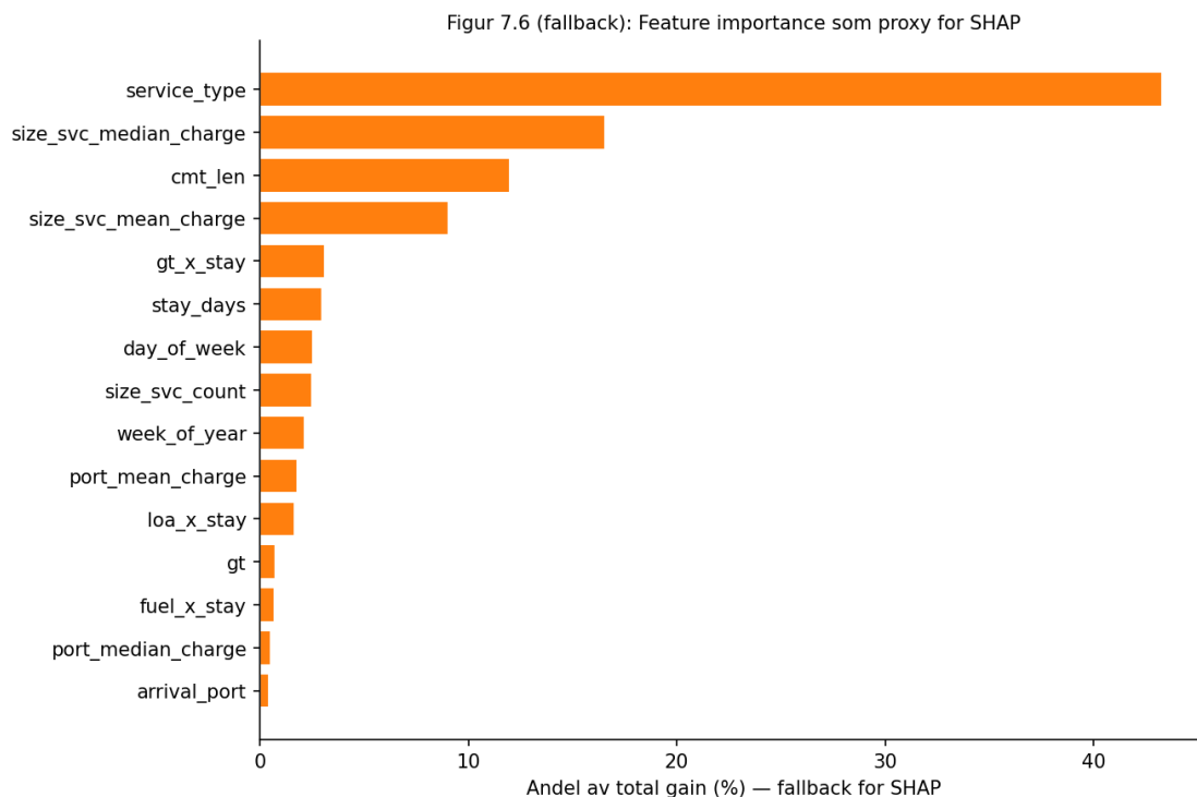
Figur 7.6: LightGBM gain-importance (fallback for SHAP, jf. § 9.7) — relativ styrke per feature i ensemblemodellen
